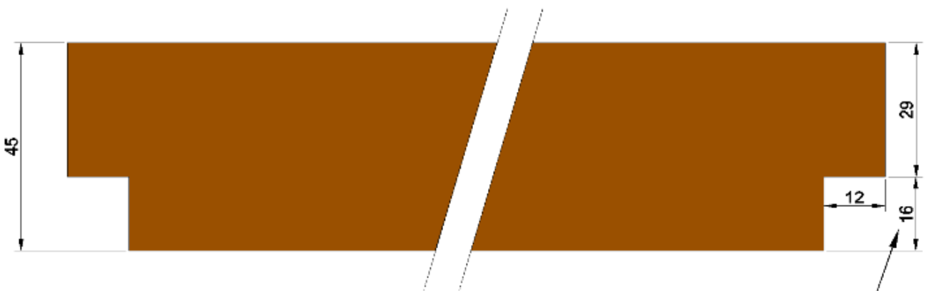
Rebate dimension for 5mm door seal
